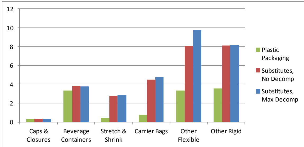
Figure ES-5. GWP Results by Category for Canadian Plastic Packaging and Substitutes (million metric tonnes CO 2 eq)
