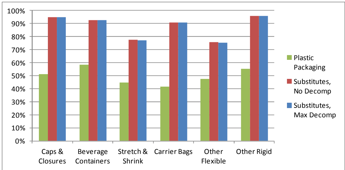
Figure 4-7. Expended Energy as a Percent of Total Energy for US Plastic Packaging and Substitutes
