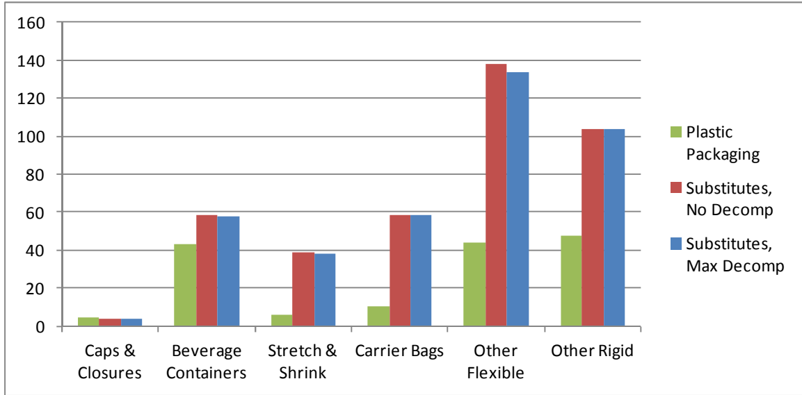
Figure 4-6. Expended Energy by Category for Canadian Plastic Packaging and Substitutes (billion MJ)
