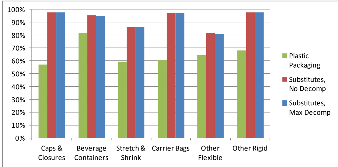
Figure 4-8. Expended Energy as a Percent of Total Energy for Canadian Plastic Packaging and Substitutes
