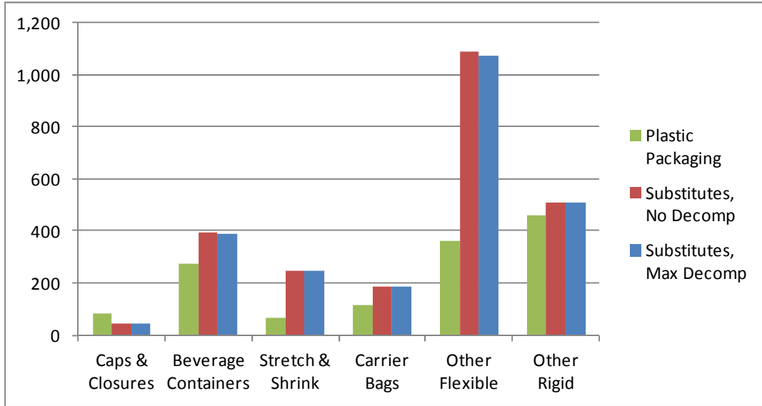
Figure 4-3. Cumulative Energy Demand by Category for US Plastic Packaging and Substitutes (billion MJ)
