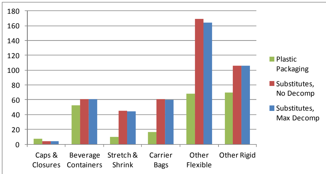
Figure 4-4. Cumulative Energy Demand by Category for Canadian Plastic Packaging and Substitutes (billion MJ)
