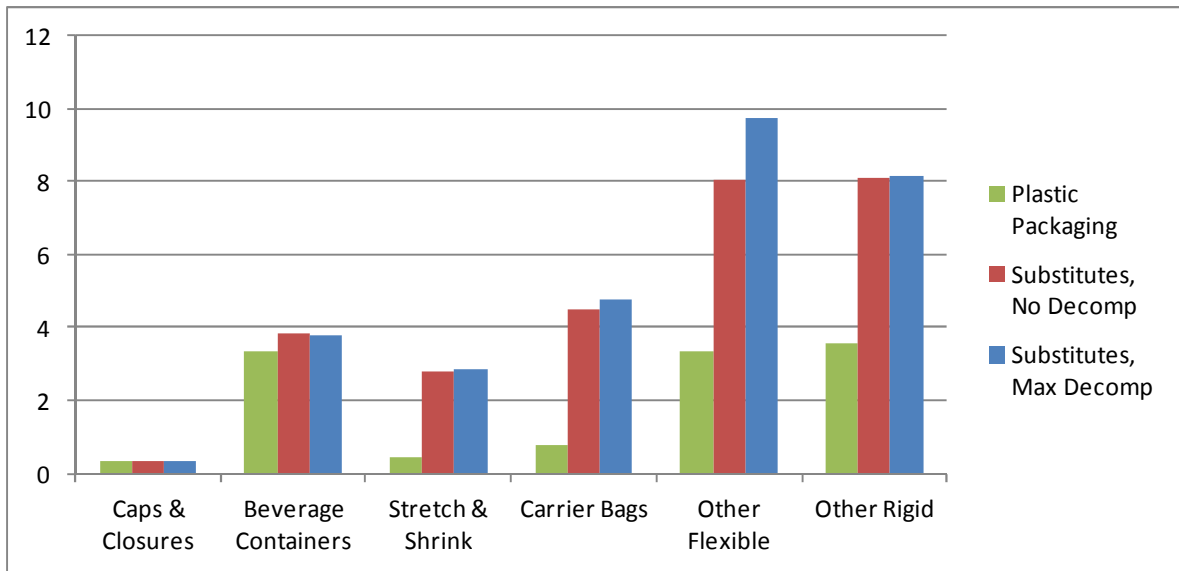
Figure 4-2. GWP Results by Category for Canadian Plastic Packaging and Substitutes (million metric tonnes CO 2 eq)
