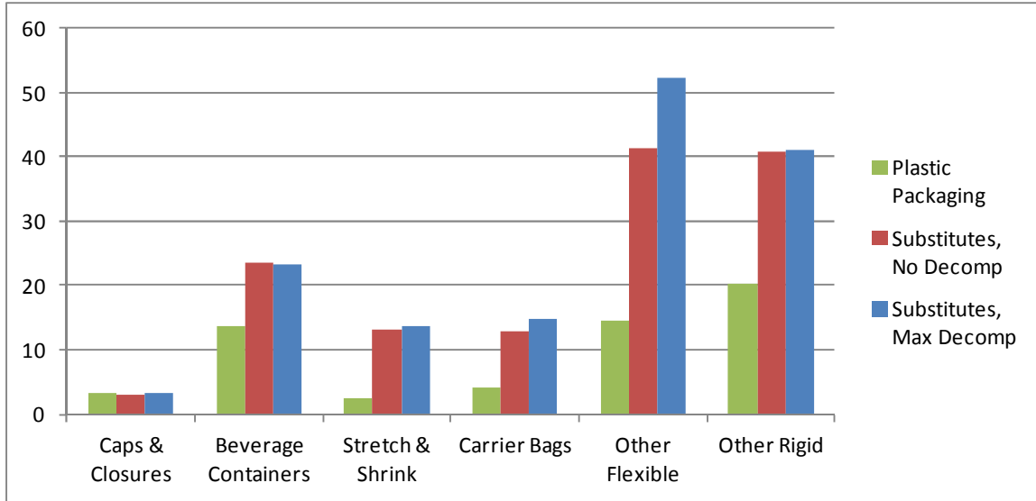
Figure ES-3. GWP Results by Category for US Plastic Packaging and Substitutes (million metric tonnes CO 2 eq)
