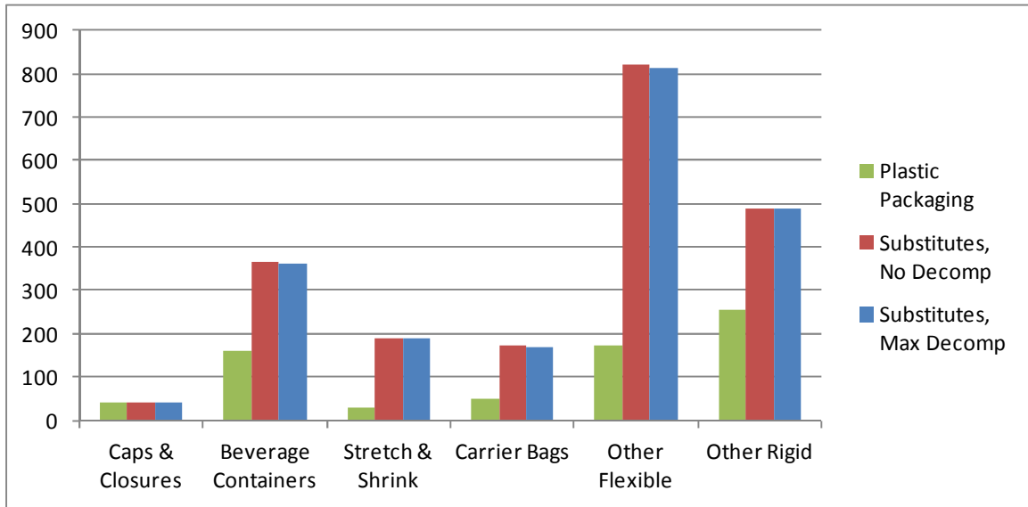
Figure 4-5. Expended Energy by Category for US Plastic Packaging and Substitutes (billion MJ)
