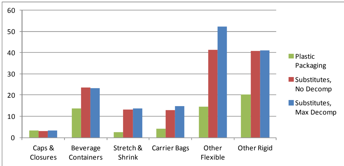
Figure 4-1. GWP Results by Category for US Plastic Packaging and Substitutes (million metric tonnes CO 2 eq)
